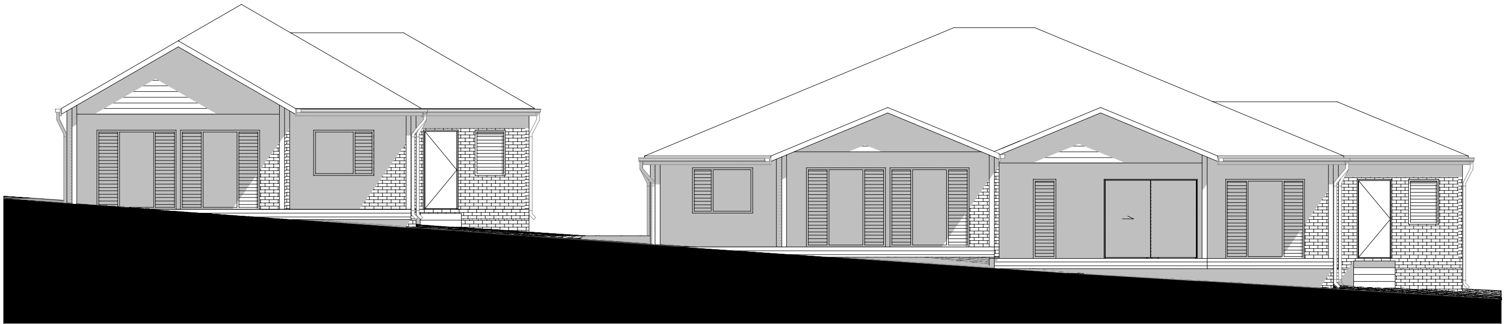
01 UNIT NORTH ELEVATION 1:100
